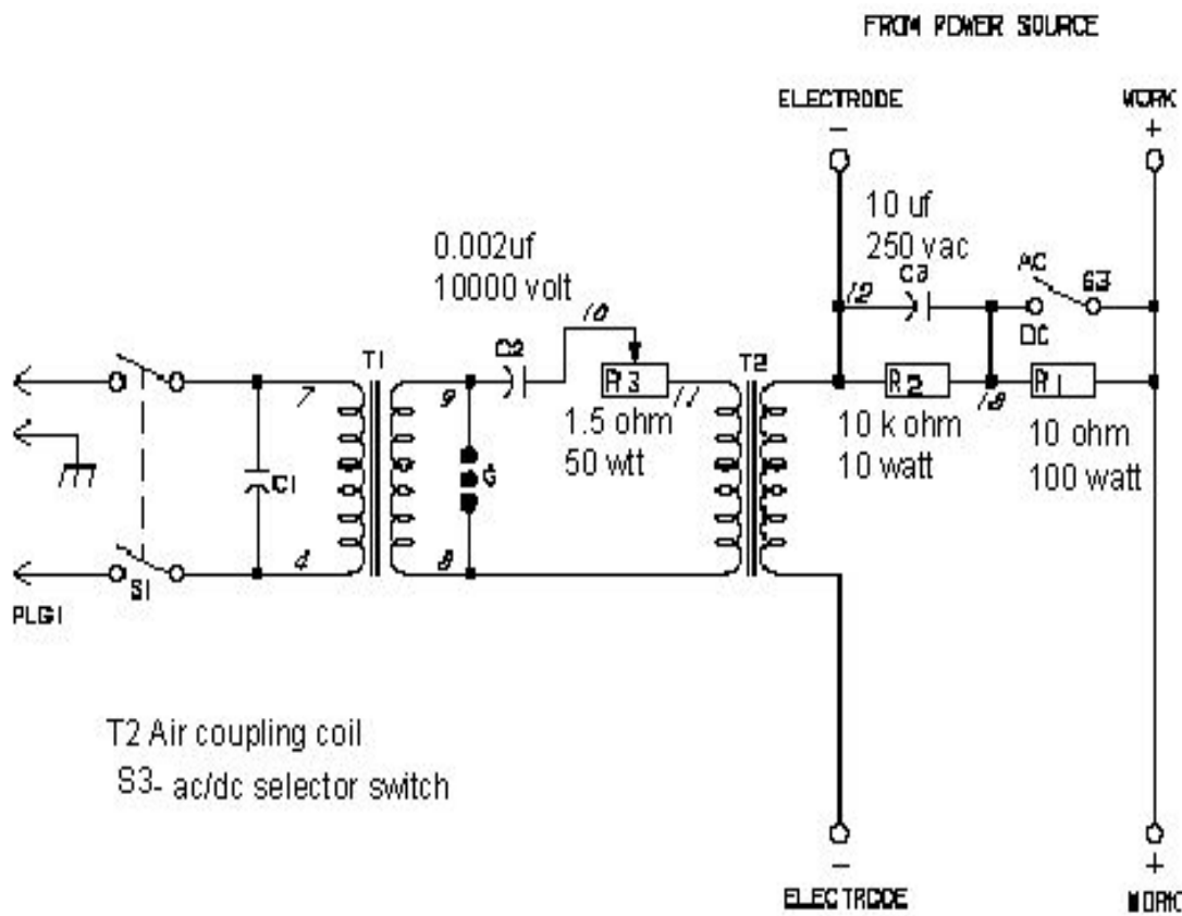
High frequency generator for Welder
